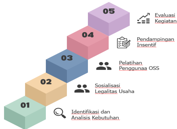
Gambar 1. Diagram Metode
