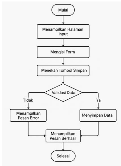
Gambar 1. Activity Diagram Form Tamu
